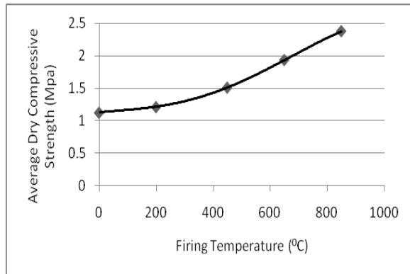
Figure 1: Effect of Firing Temperature on Compressive Strength of Samples
