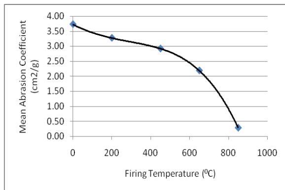
Figure 2: Effect of Firing Temperature on the Abrasive Coefficient of Samples
