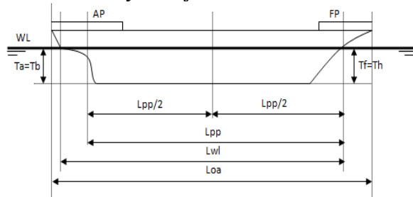
Fig.1: Longitudinal Shape of the Vessel
