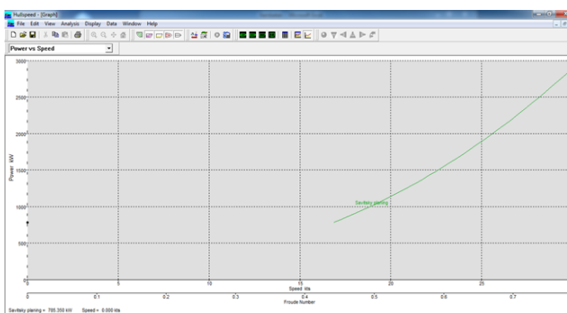
Fig.11: The Graph of Resistance vs Speed T=1.50
