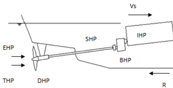
Fig.3: Propulsion System of the Vessel
