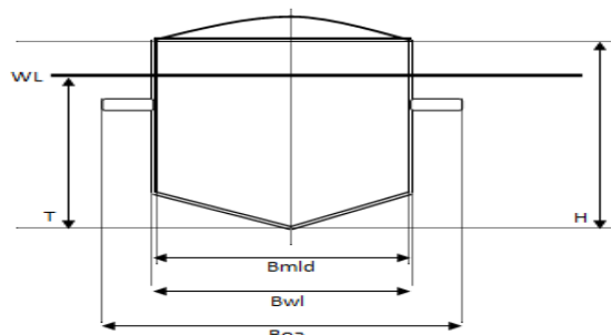
Fig.2: Cross-sectional Shape of the Vessel
