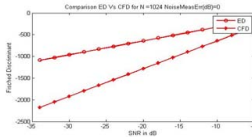
Fig.4 Graph “SNR Vs Fischer Discriminant” comparison for ED and CFD
